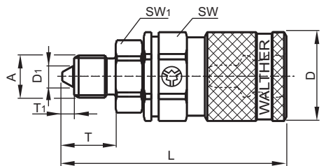
Муфта с клапаном / Self sealing coupling (with valve) HP-004-0-XX002-AAAZ-Y46
